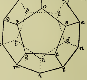
Irregular rhombic dodecahedron
